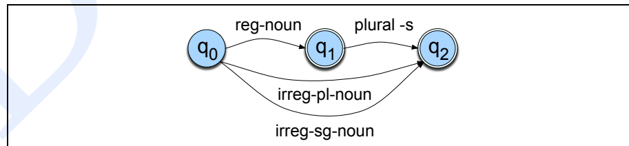
Figure 3.3 A finite-state automaton for English nominal inflection.
