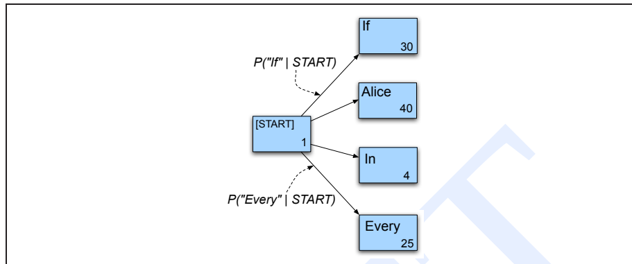
Figure 10.8 The beginning of the search for the sentence If music be the food of love . At this early stage Alice is the most likely hypothesis. (It has a higher score than the other hypotheses.)
